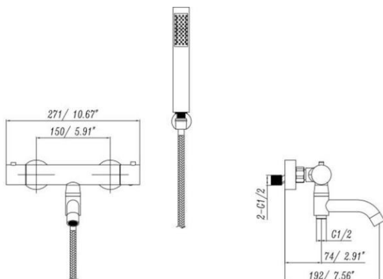
Dimensions scheme [mm / inches]:
